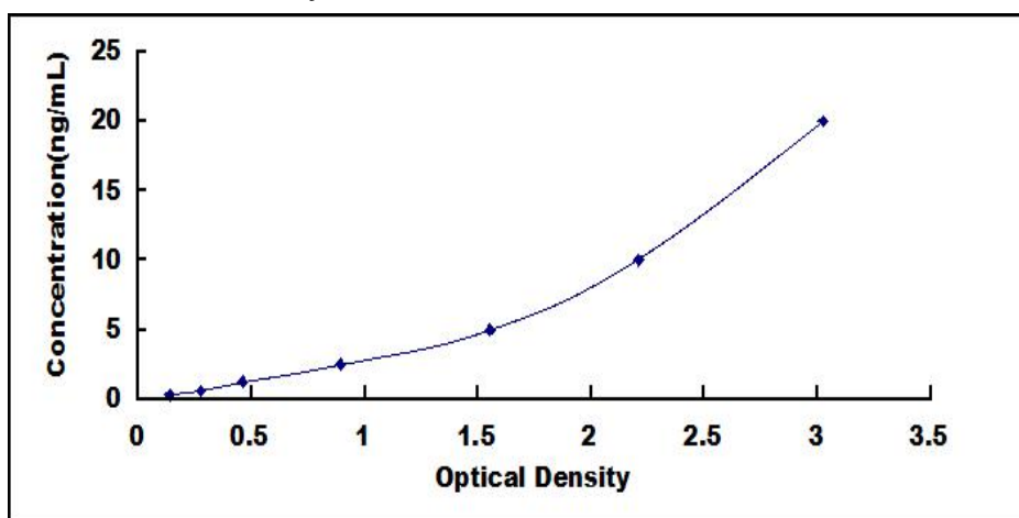
Typical Standard Curve for CST5 ELISA.
