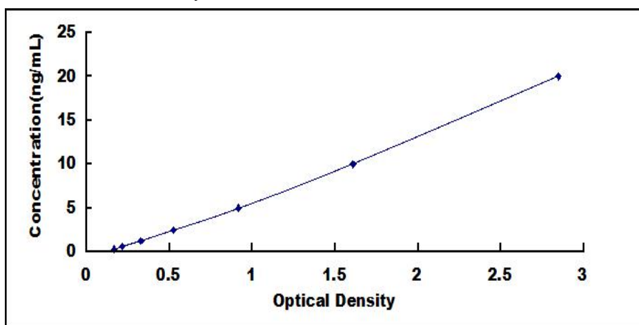
Typical Standard Curve for DHX36 ELISA.
