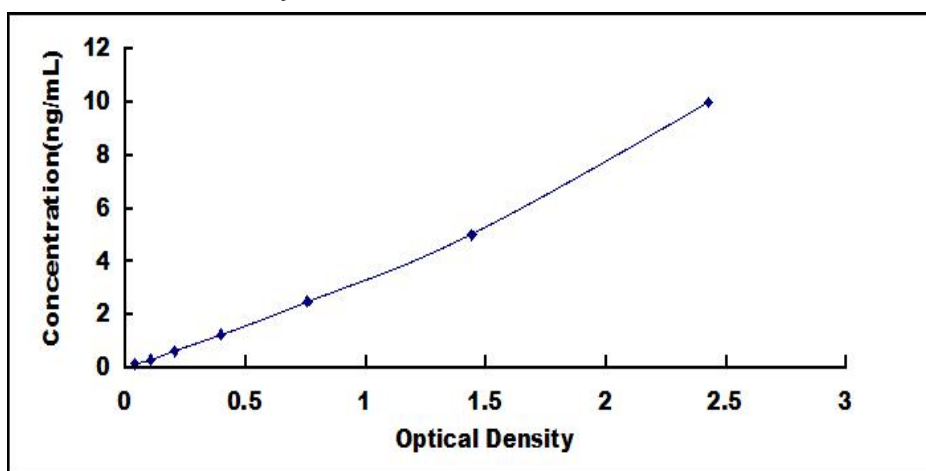
Typical Standard Curve for MRPL53 ELISA.
