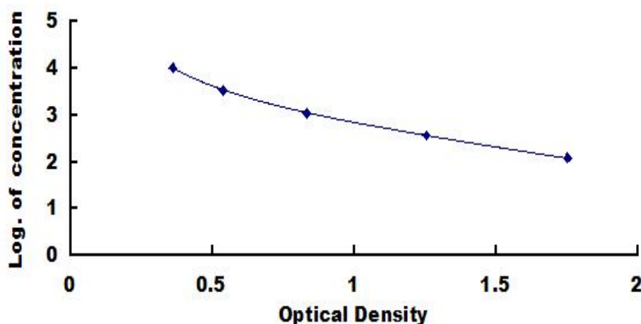
Typical Standard Curve for PCr ELISA.
