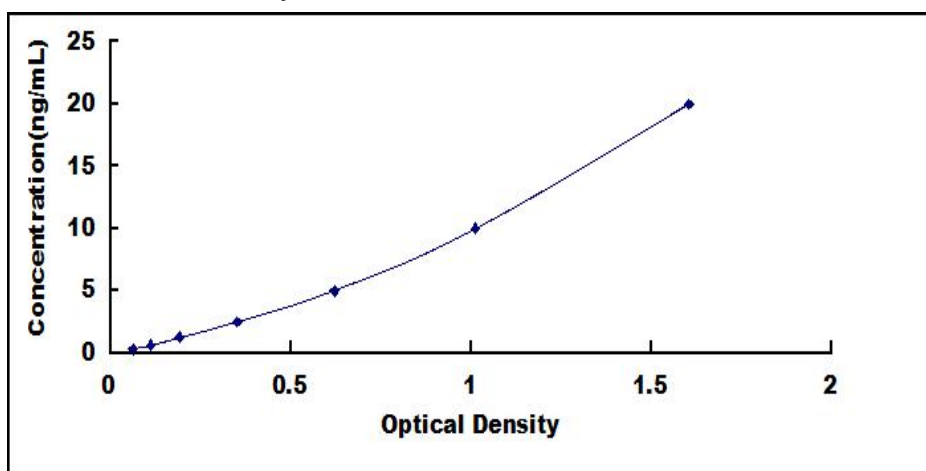
Typical Standard Curve for SEMA5B ELISA.
