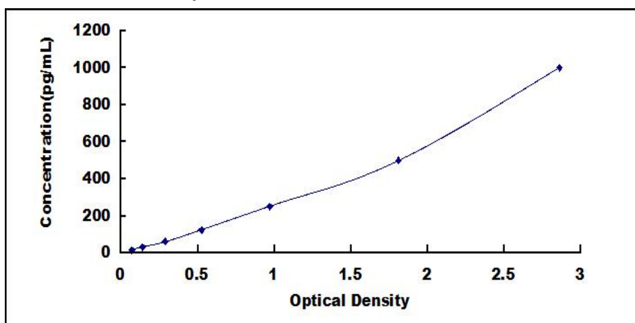
Typical Standard Curve for DR5 ELISA.
