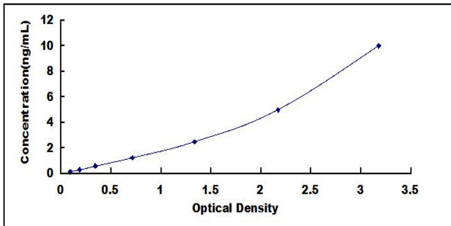
Typical Standard Curve for NOV ELISA.
