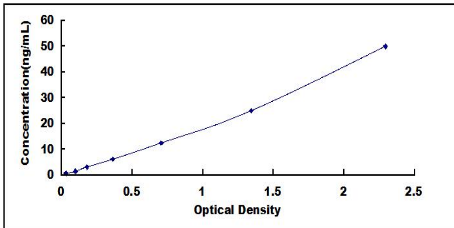
Typical Standard Curve for TBG ELISA.
