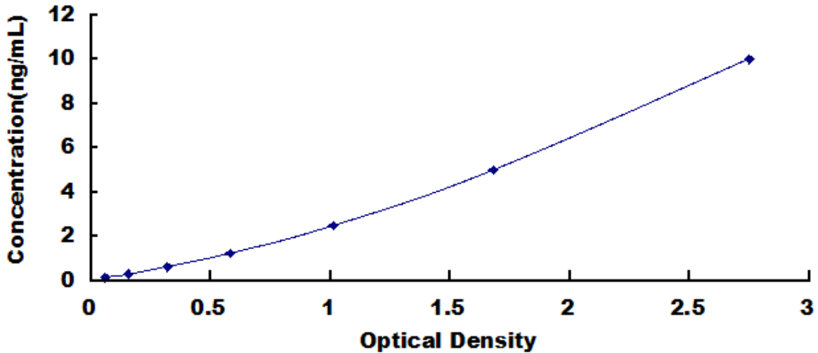
Typical Standard Curve for PDK4, Human ELISA.
