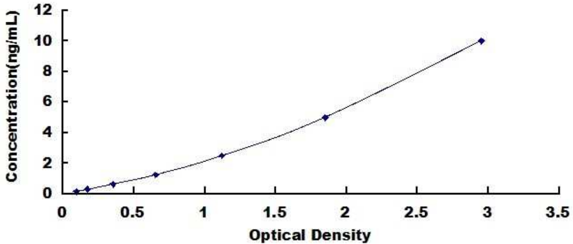
Typical Standard Curve for ANGPTL3, Porcine ELISA.
