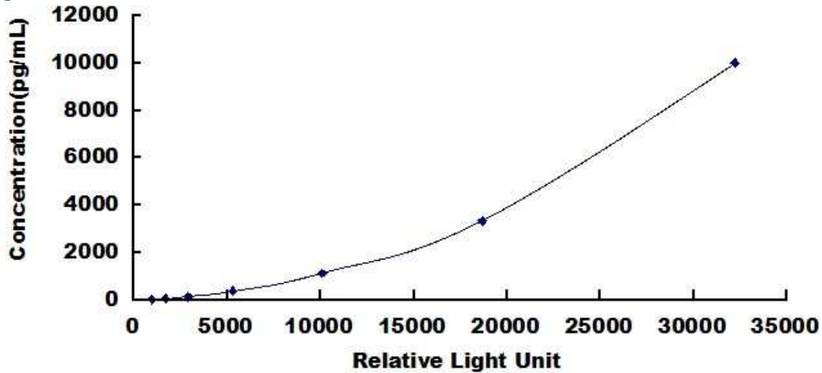
Typical Standard Curve for SORT1, Human CLIA.
