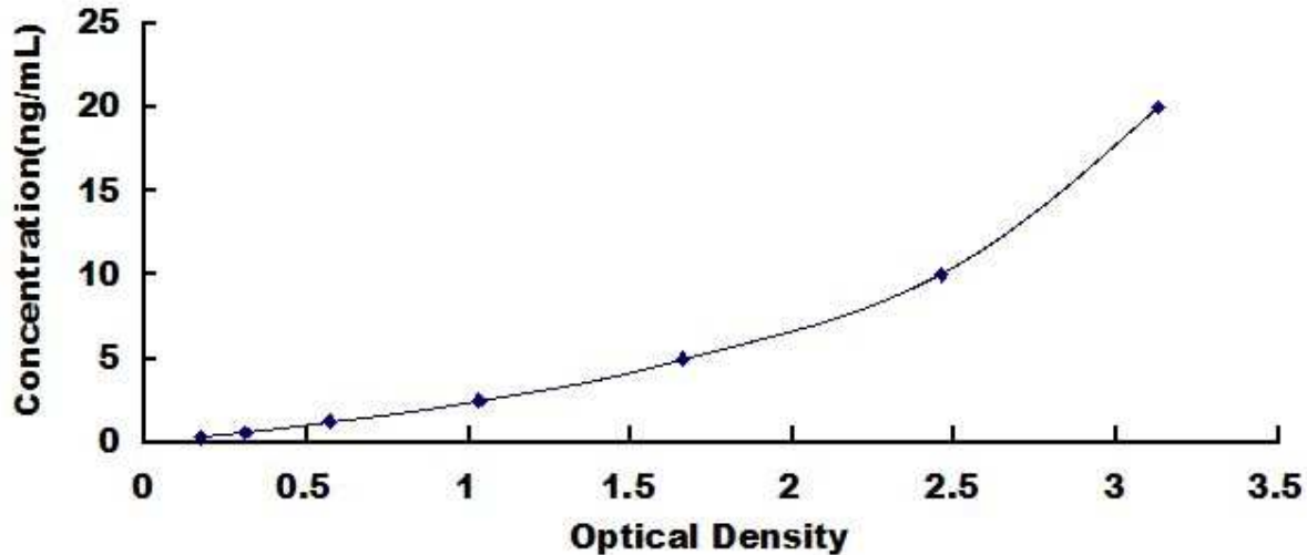
Typical Standard Curve for SMPD3, Rat ELISA.
