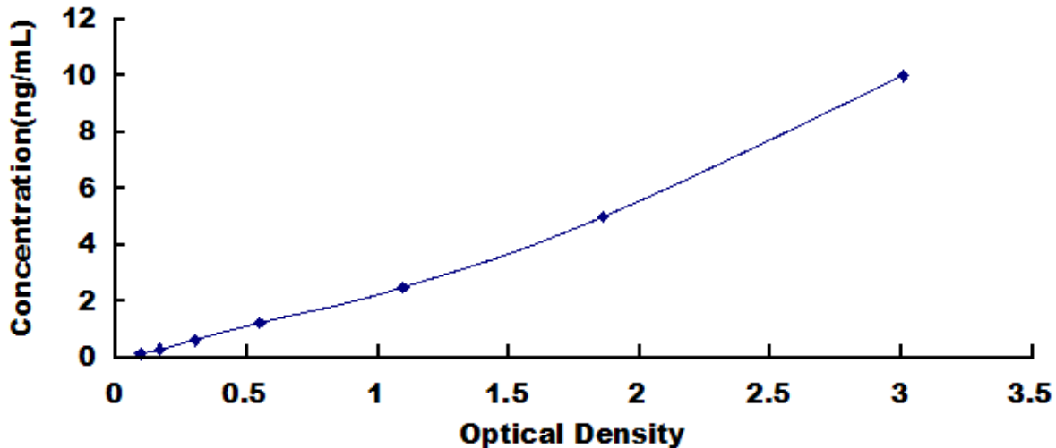
Typical Standard Curve for ATF6, Rat ELISA.
