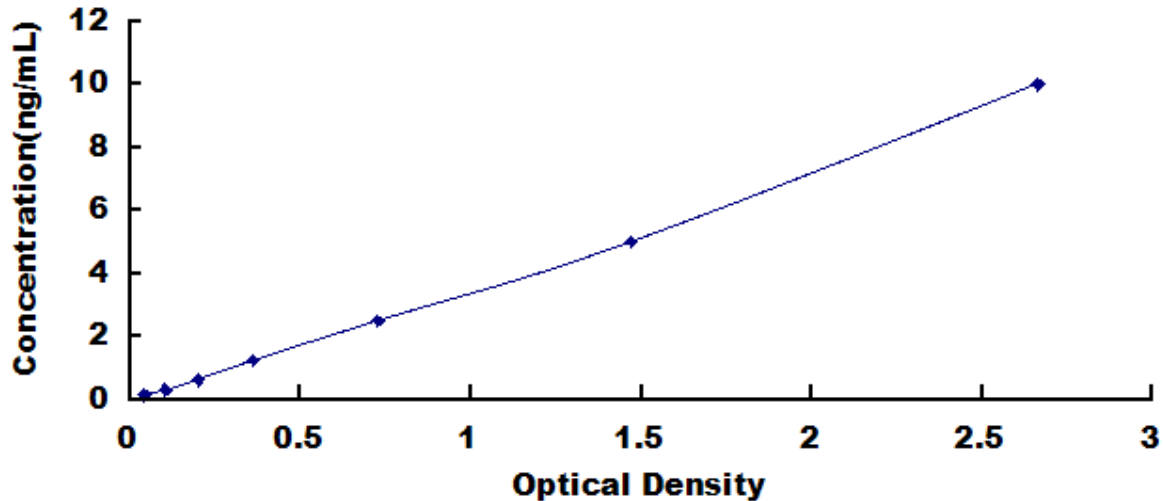
Typical Standard Curve for ASAH2, Rat ELISA.
