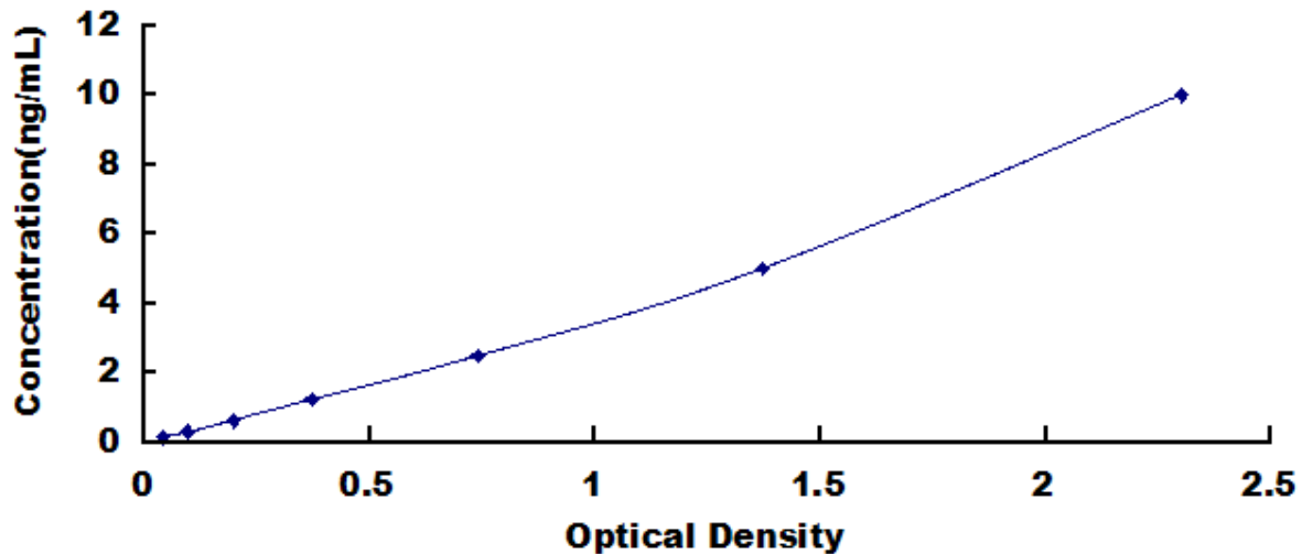
Typical Standard Curve for IRF4, Mouse ELISA.
