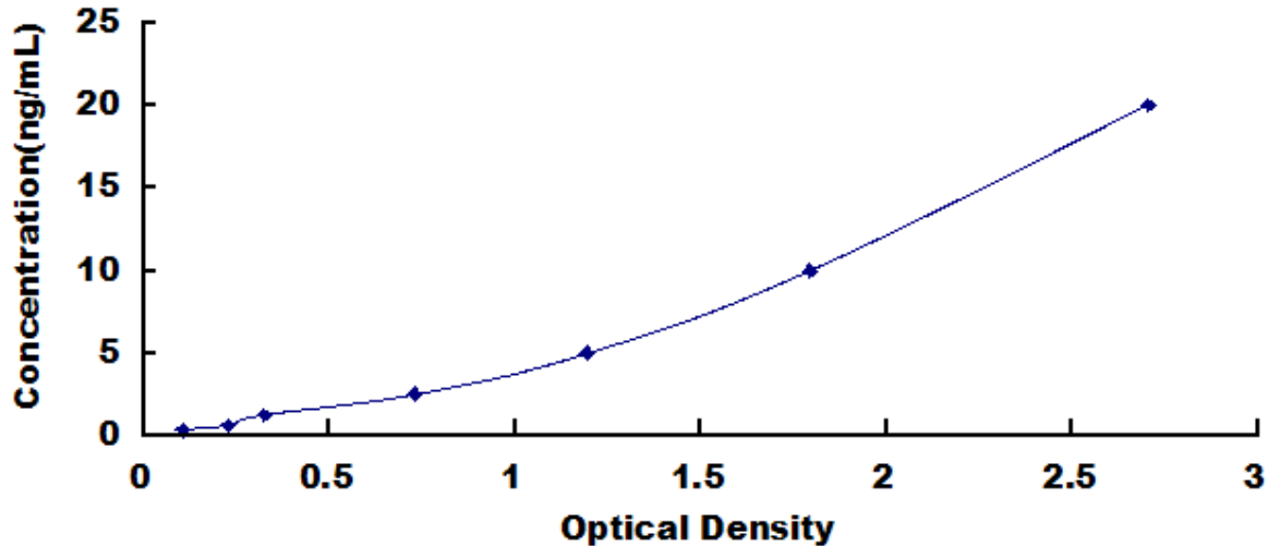
Typical Standard Curve for RYR2, Mouse ELISA.
