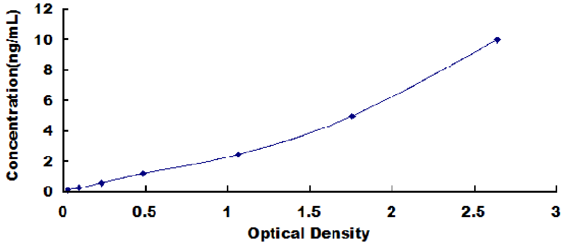
Typical Standard Curve for CTSH, Rat ELISA.
