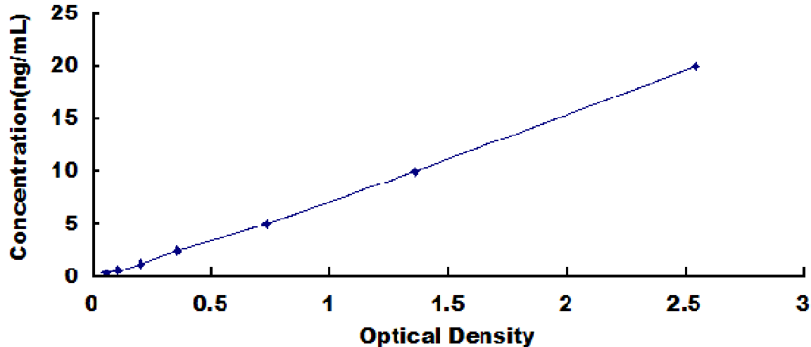
Typical Standard Curve for FOXO3, Rat ELISA.
