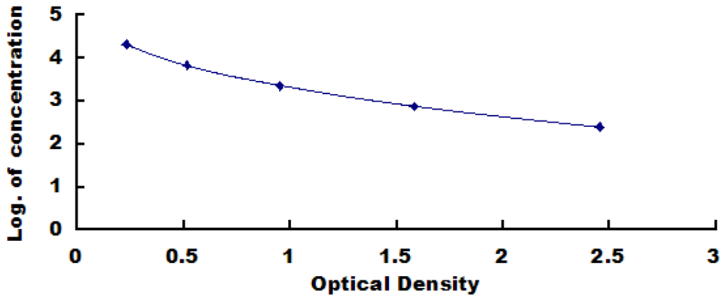
Typical Standard Curve for IgG2, Bovine ELISA.
