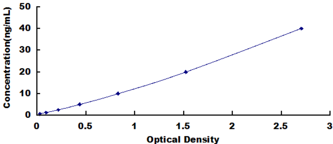
Typical Standard Curve for KLK8, Mouse ELISA.
