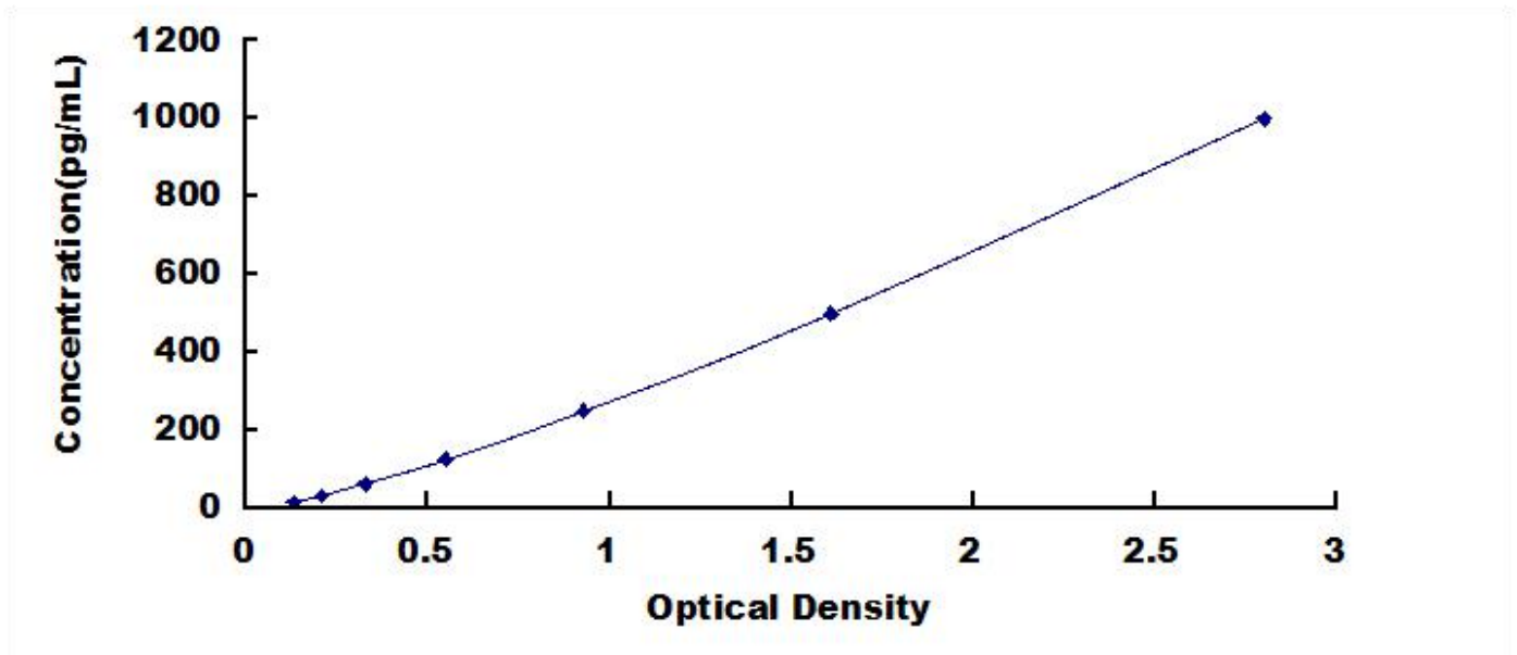
Typical Standard Curve for VEGFA, Simian ELISA.
