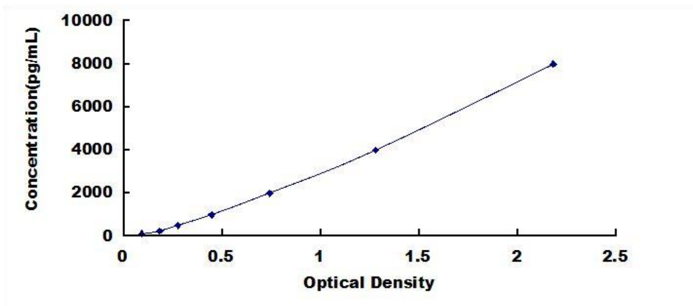
Typical Standard Curve for HSP47, Human ELISA.
