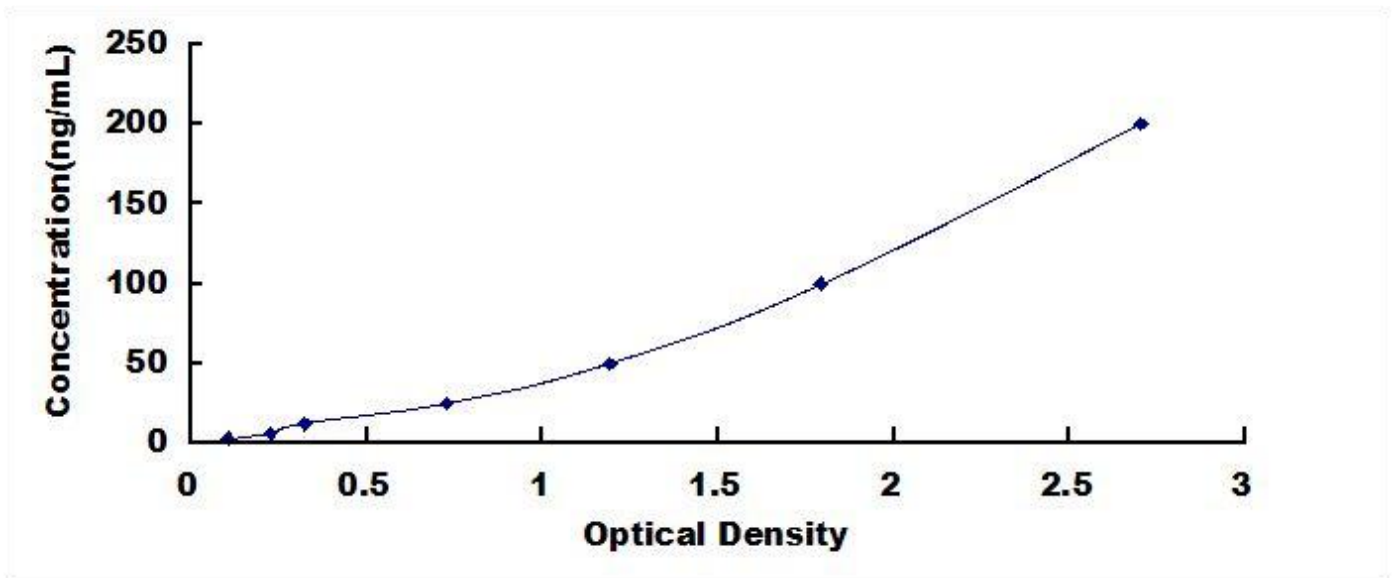
Typical Standard Curve for LDH, Human ELISA.
